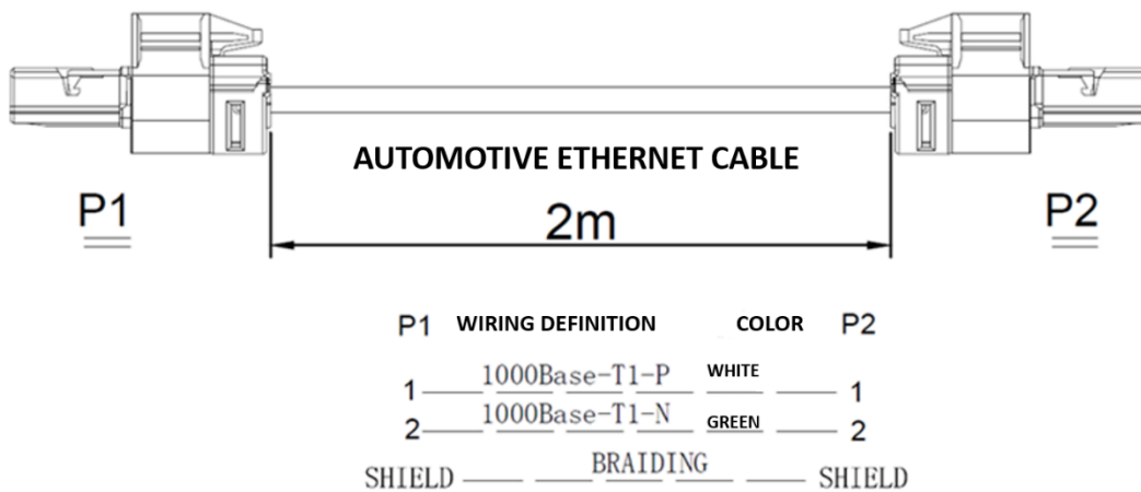
Figure 2.2 The 2-Pin Automotive Ethernet Cable
