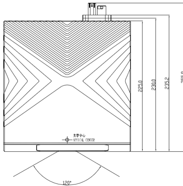
Figure 1.4 Optical Centre of the LS25D Lidar
