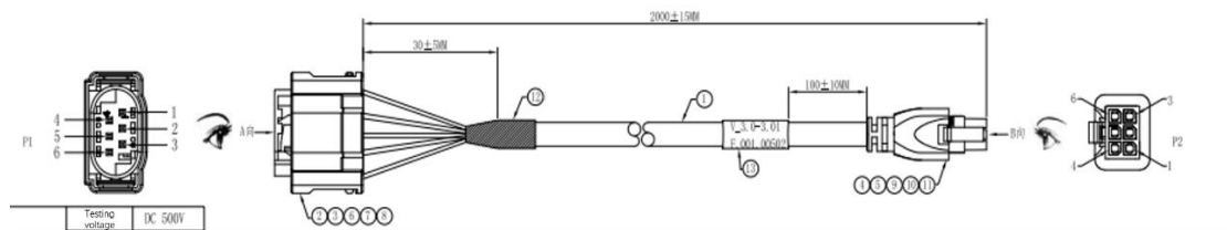
Figure 2.1 The 6-Pin Power Cord (GPS Time Service)
