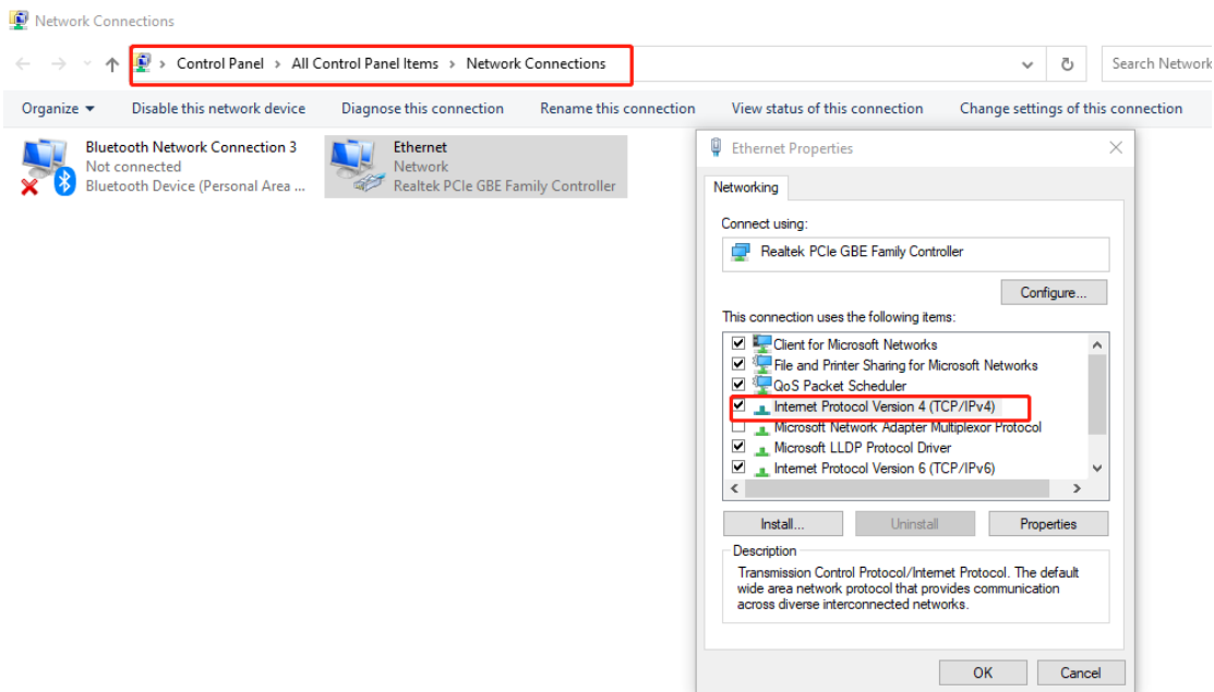
Figure 4.4 Network Connections
