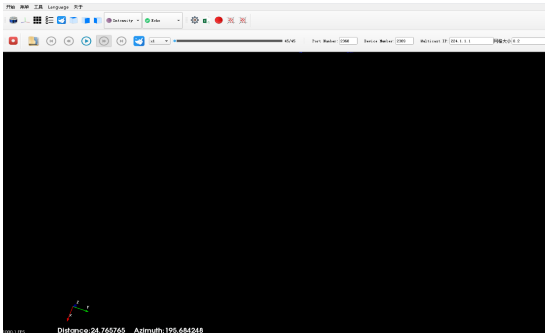
Figure 4.2 Initial Interface
