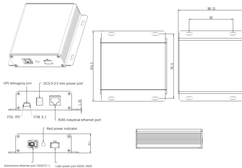
Figure 2.3 Interface Box of LS25D
