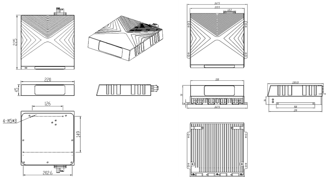
Figure 1.2 LS25D Lidar Mechanical Drawing (left: bare lidar; right: with cooling base)
